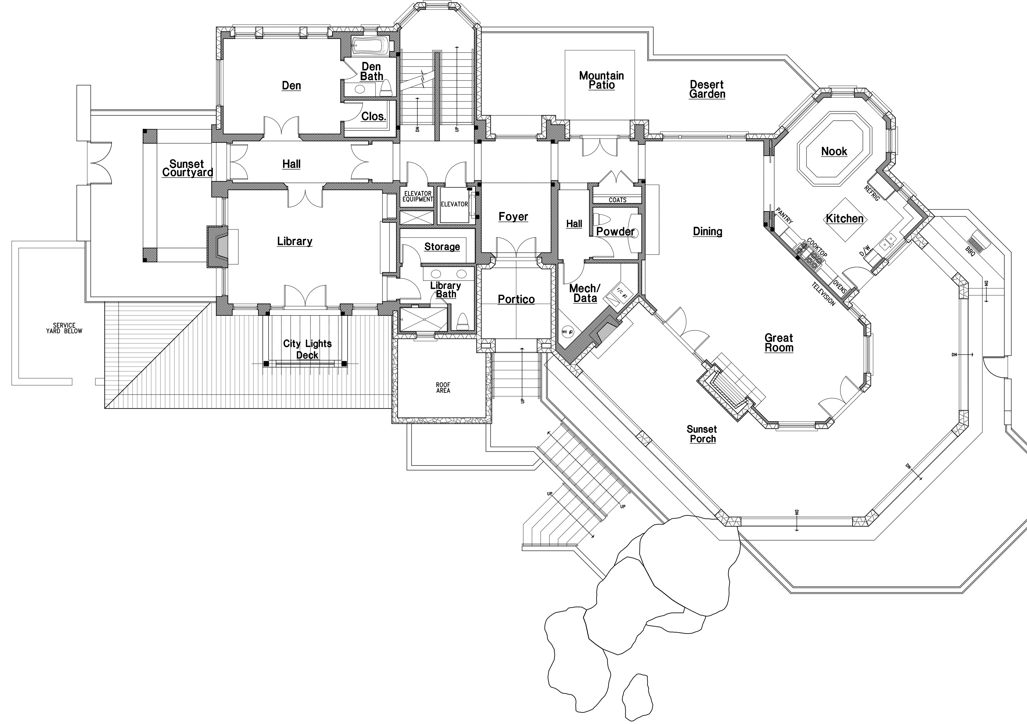
GUEST HOUSE ENTRY FLOOR PLAN
